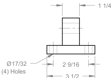
Eye Bracket #08040368
